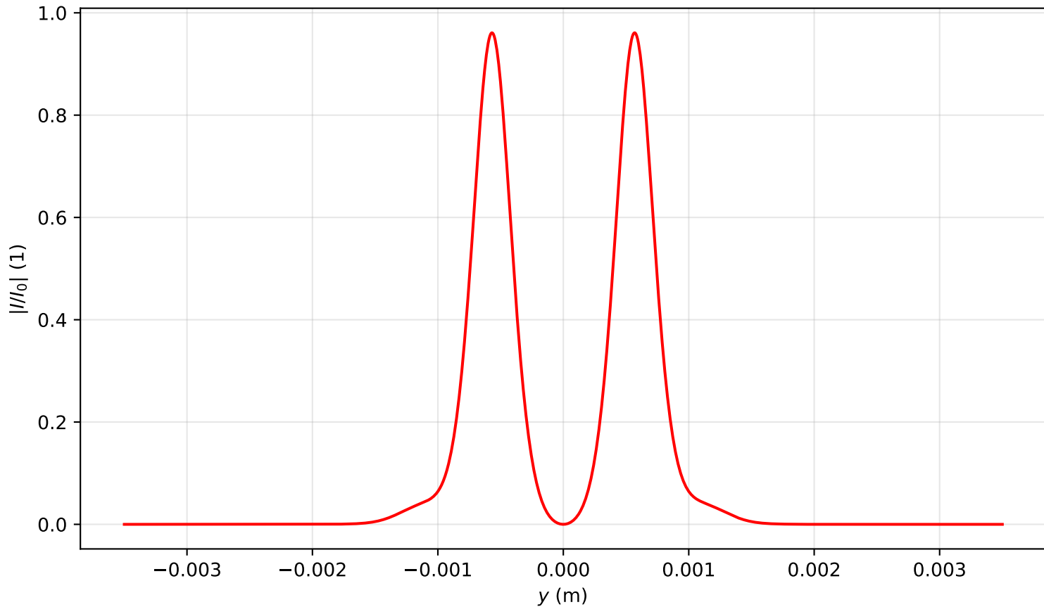
Intensity profile I(x=0, y, z=0.796)/I_0 , \text{Pin}=5.0\text{Pcr} , artificial time
